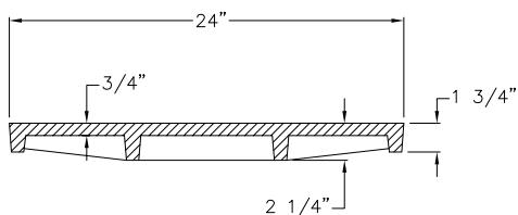
COVER SECTION
