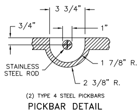
PICKBAR DETAIL
