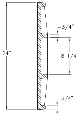
COVER SECTION
